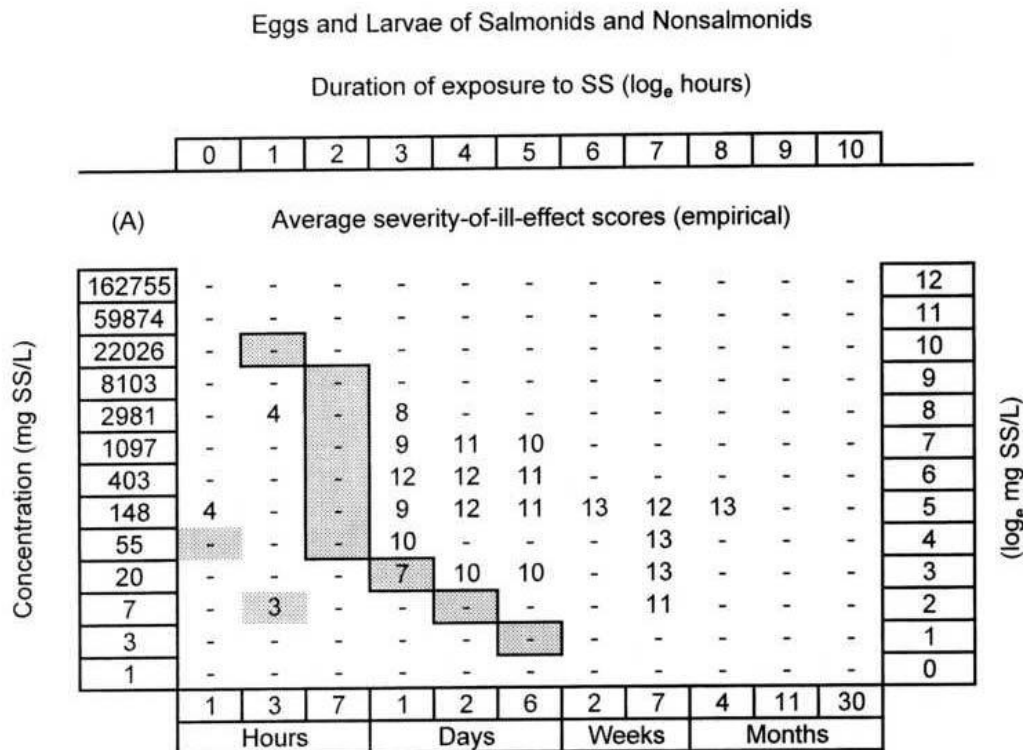
FIGURE 4.—Empirical severity-of-ill-effect scores for eggs and larvae of salmonids and nonsalmonids (freshwater and estuarine, group 4) and scores (with half-95% confidence intervals) predicted by model (4). Conventions are those of Figure 1, except the model (B, upper matrix) recognized no threshold of sublethal effects.
