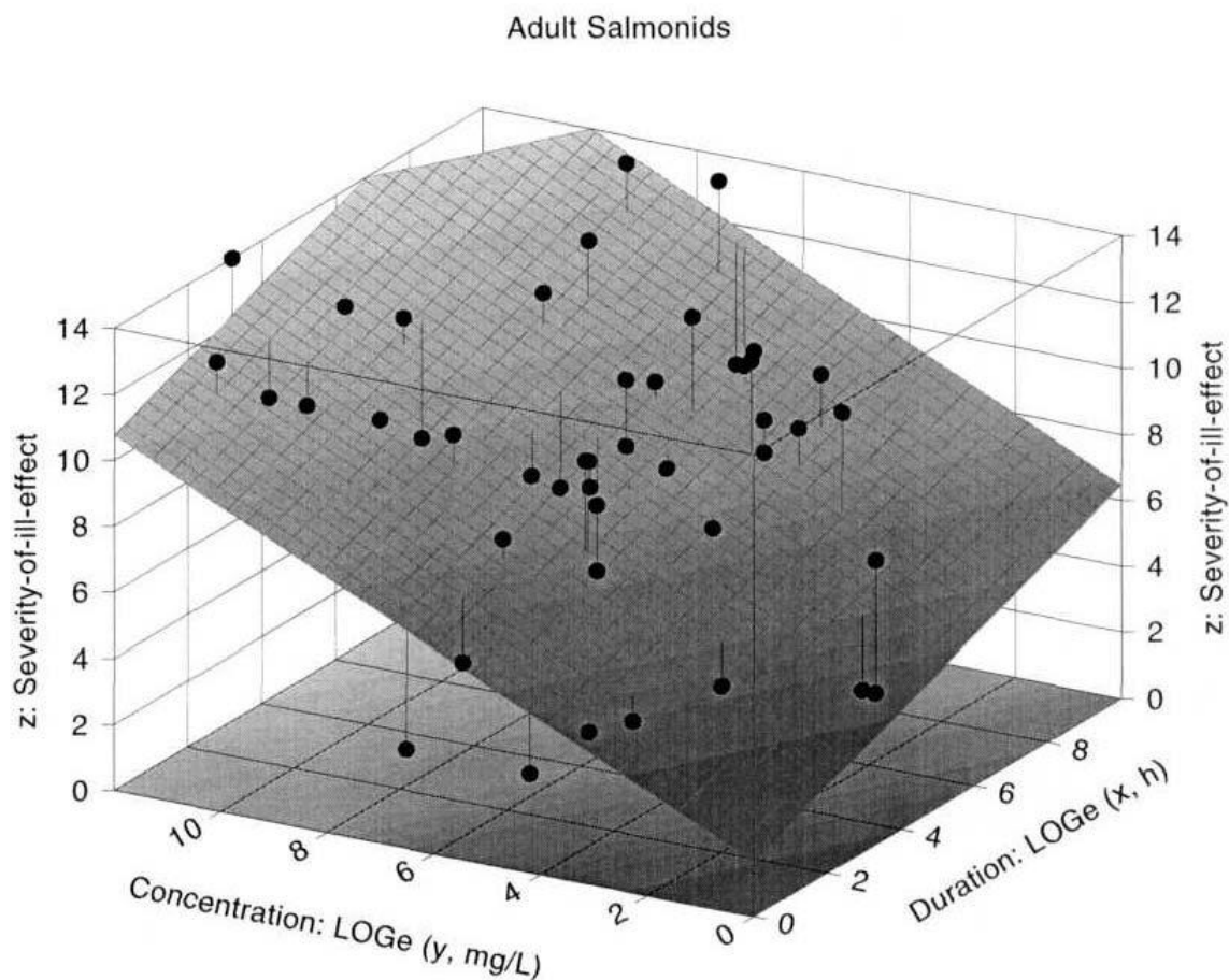
FIGURE 8.—Dose–response surface describing the severity of ill effect for adult salmonids (freshwater, group 2) as a function of suspended sediment concentration and duration of exposure (model 2): z = 1.6814 + 0.4769(\log_e x) + 0.7565(\log_e y) .
