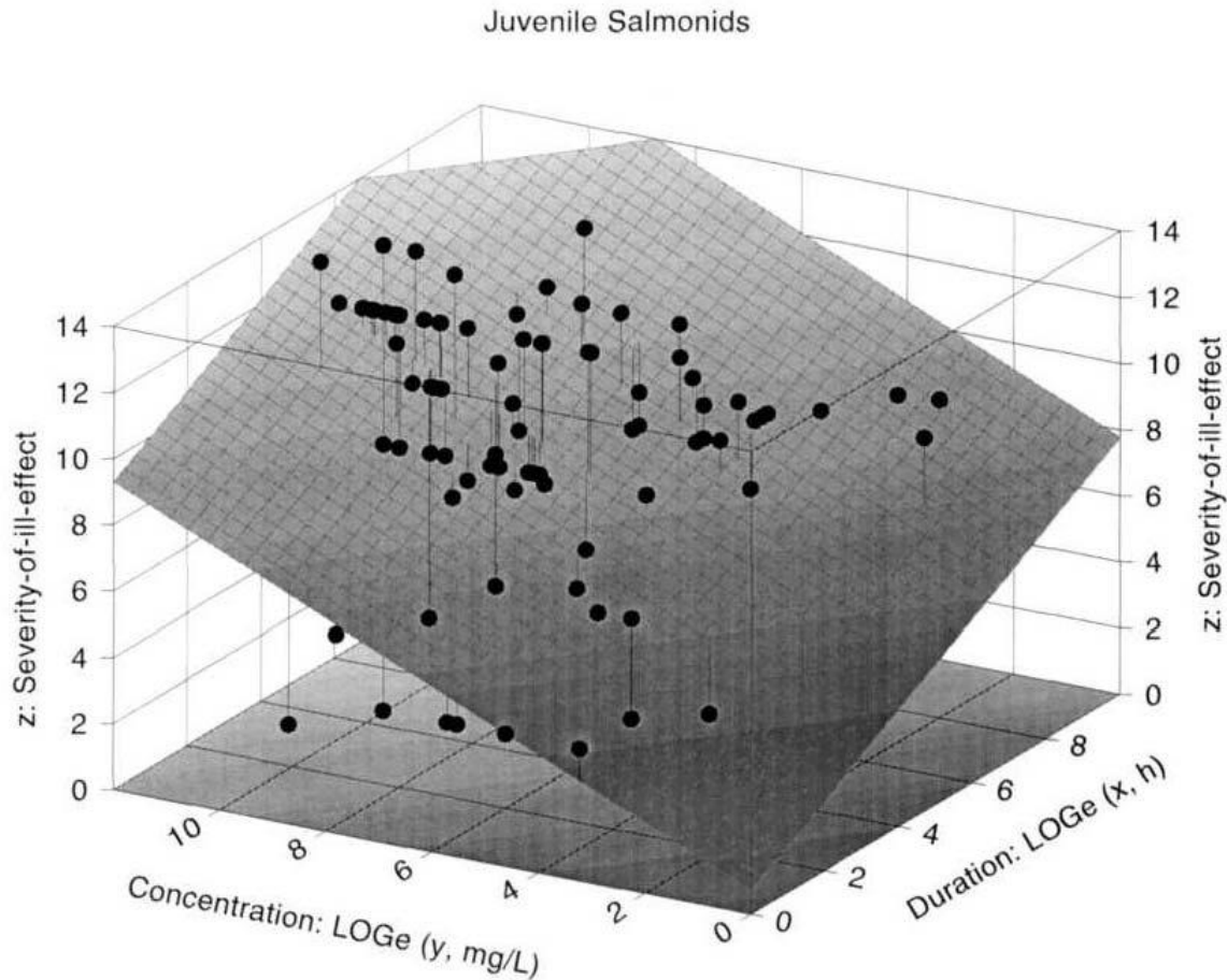
FIGURE 9.—Dose–response surface describing the severity of ill effect for juvenile salmonids (freshwater, group 3) as a function of suspended sediment concentration and duration of exposure (model 3): z = 0.7262 + 0.7034(\log_e x) + 0.7144(\log_e y) .
